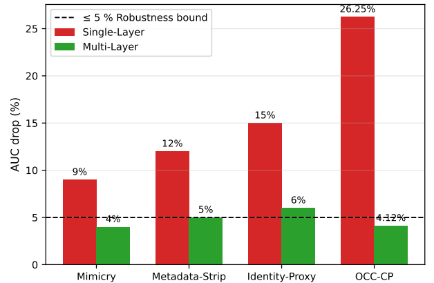
Figure 8: AUC Drop vs Robustness Bound ( \leq 5\% ) Across Attacker Vectors.
