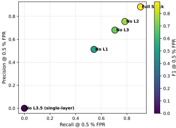
Figure 6: Pareto Precision-Recall Frontier Across Layer Ablations on D5 Hold-Out.
