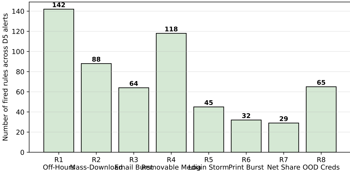
Rule-Family Activation Profile across 583 detected alerts
