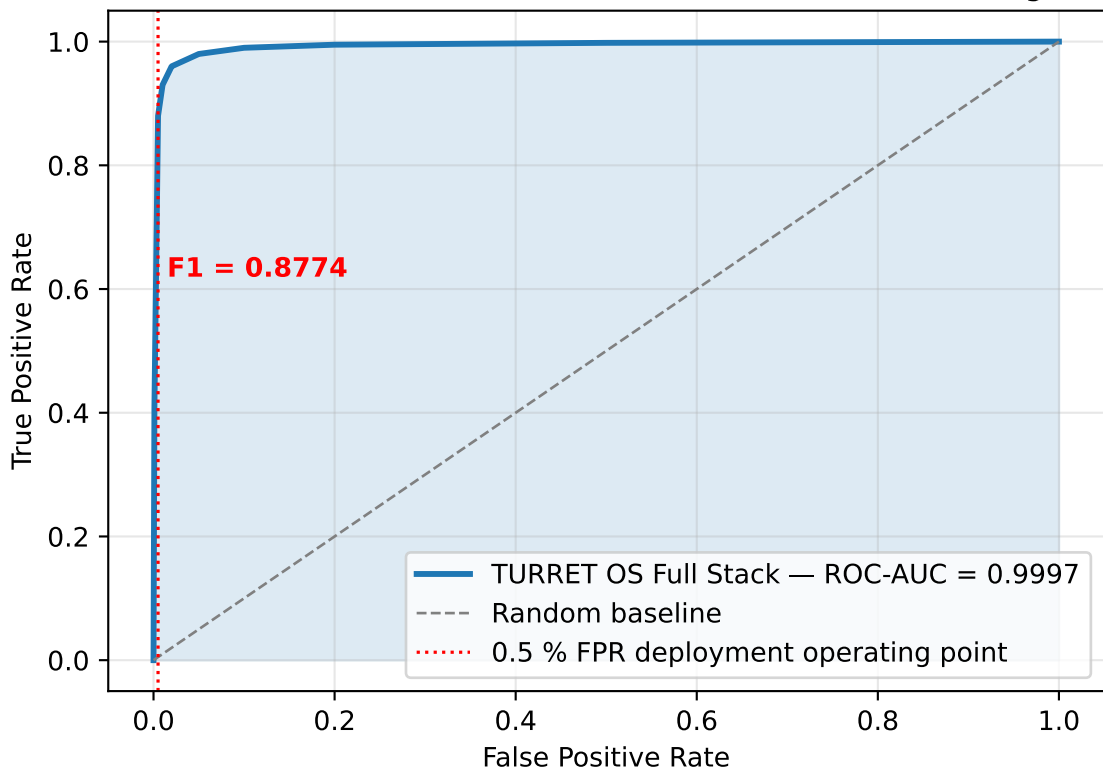
ROC Curve — TURRET OS on D3 TSEC (60-30-10 chronological)
