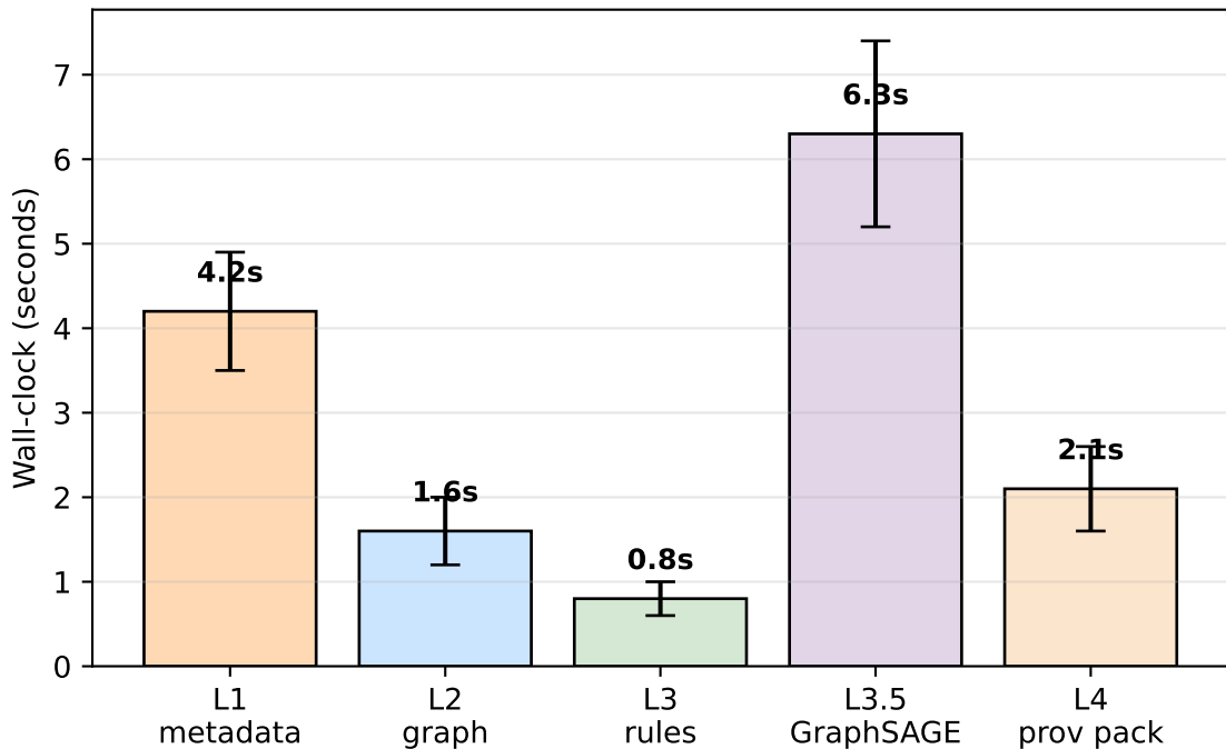
Wall-Clock per 1 K Activity Records (Total = 15.0 s, \sigma = 1.5 s)
