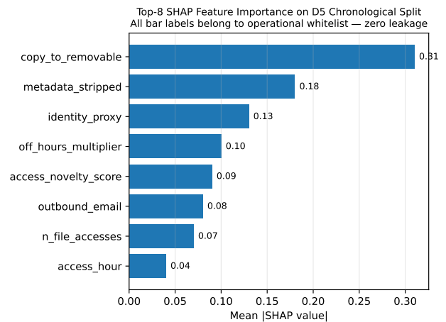
Figure 6: Top-8 SHAP Feature Importance on D5 Chronological Split (Verified Operational Whitelist).
