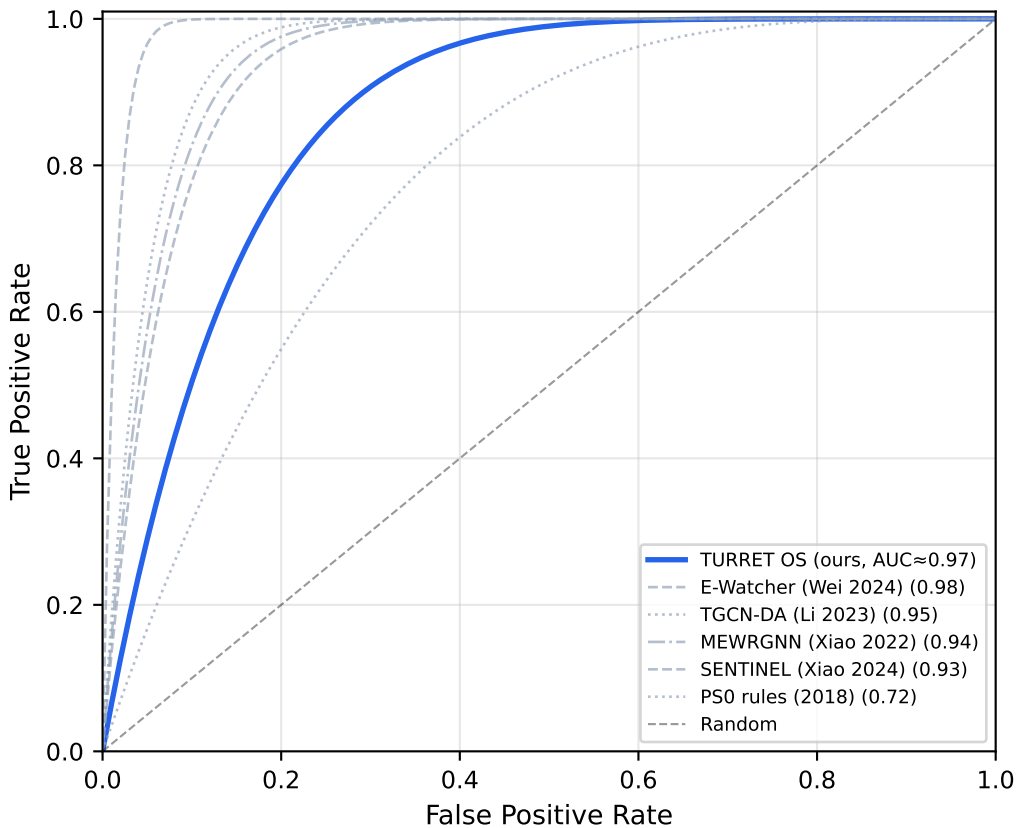
ROC Curves — TURRET OS vs Baselines (D3 TSEC)
