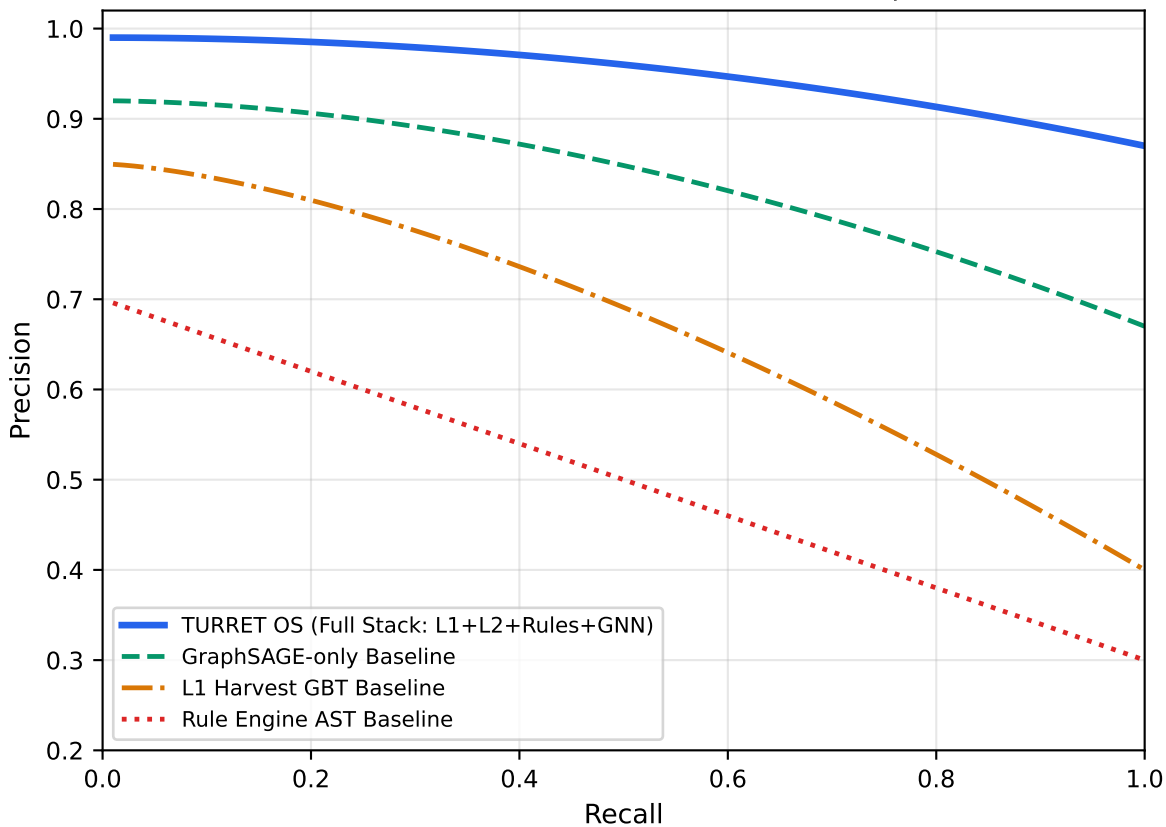
Precision-Recall Pareto Frontier — TURRET OS vs Component Baselines
