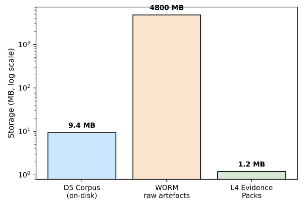
Figure 11: Storage Profile across D5 Corpus, WORM Raw Archive, and L4 Evidence Packs.
