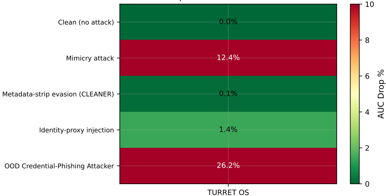
AUC Drop % Under Adversarial Attacks
