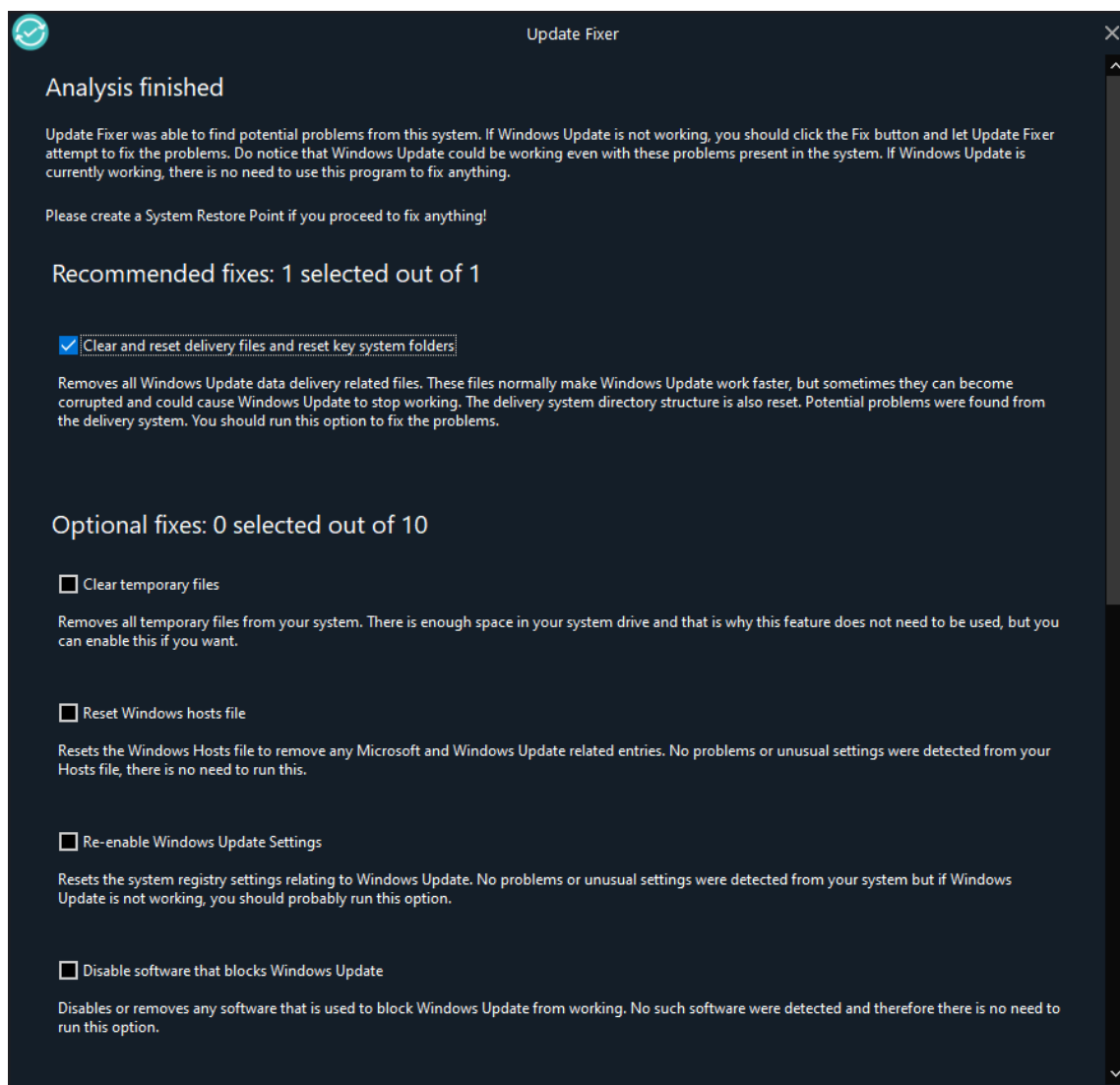
Screenshot 2 - The program showing what is wrong with your Windows Update and what it recommends you to do. These options are presented based on analysis of your computer.
