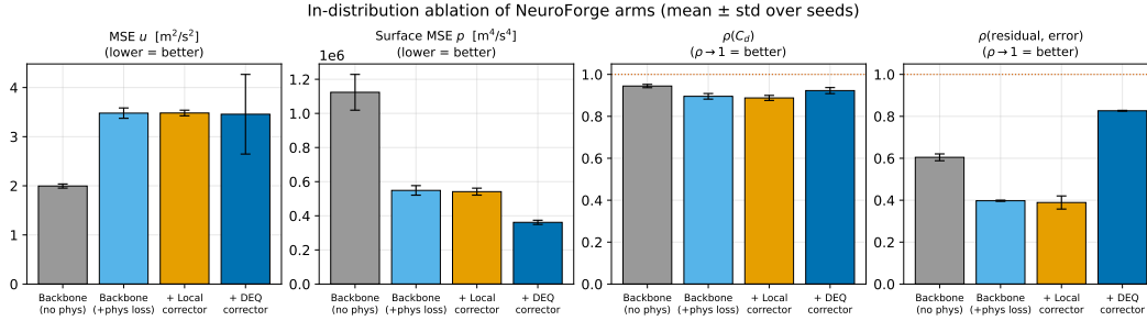
Figure 3: In-distribution ablation (Table 3): the DEQ corrector lifts the trust signal (0.40 \rightarrow 0.83) and surface fidelity while regressing volume mse_v/mse_p .
