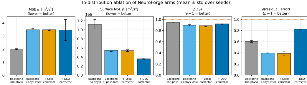
Figure 1: In-distribution ablation (Table 3): the DEQ corrector lifts the trust signal ( 0.40 \rightarrow 0.83 ) and surface fidelity while regressing volume \text{mse}_v/\text{mse}_p .
