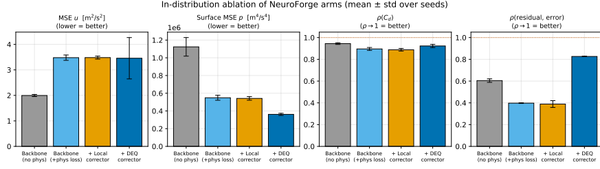
Figure 1: In-distribution ablation (Table 7): the DEQ corrector lifts the trust signal ( 0.40 \rightarrow 0.83 ) and surface fidelity while regressing volume \text{mse}_v/\text{mse}_p .
