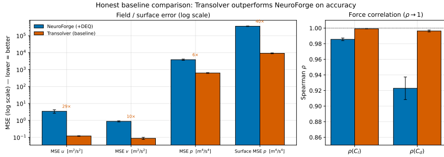
Figure A.7: Matched-budget baseline (Table 1): the grid backbone trails Transolver \sim 4 – 60\times across channels (no competitiveness claim).
