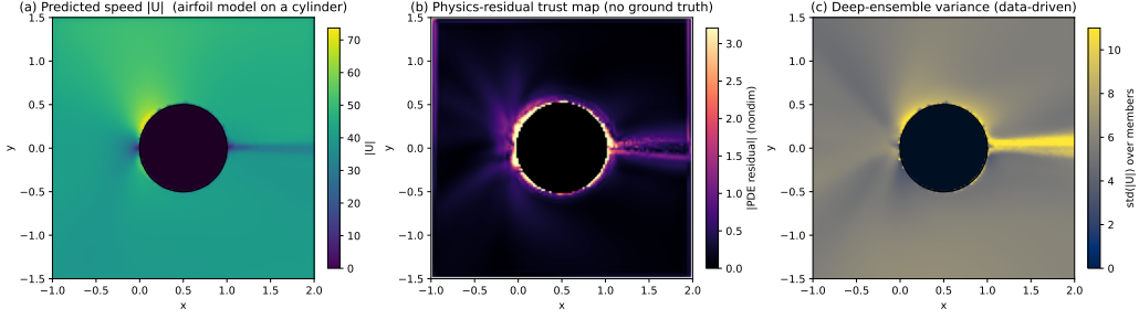
Figure A.8: Cross-geometry OOD (qualitative): an airfoil-trained model on a cylinder. (a) predicted speed (visibly broken); (b) the physics-residual map (no ground truth used), elevated field-wide; its bright near-body ring is a generic no-slip-wall feature common to all bodies, not an OOD localiser; (c) deep-ensemble variance. The OOD signal is the field-wide residual magnitude — \approx 7\times higher than in-distribution airfoils in the far field, away from any wall (subsection 4.6)—not its spatial concentration.
