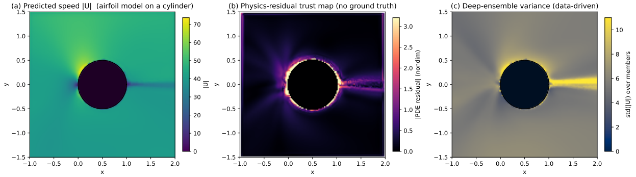
Figure 7: Cross-geometry OOD (qualitative): an airfoil-trained model on a cylinder. (a) predicted speed; (b) the physics-residual trust map localises on the body surface where the field violates the PDE (no ground truth used); (c) deep-ensemble variance from the five members (the uncorrected ensemble, the source of \sigma ) does not localise there. Physics flags where the geometry breaks the equations; data-driven variance does not. The residual is a local-violation detector—note the smoothly-wrong wake stays dark.
