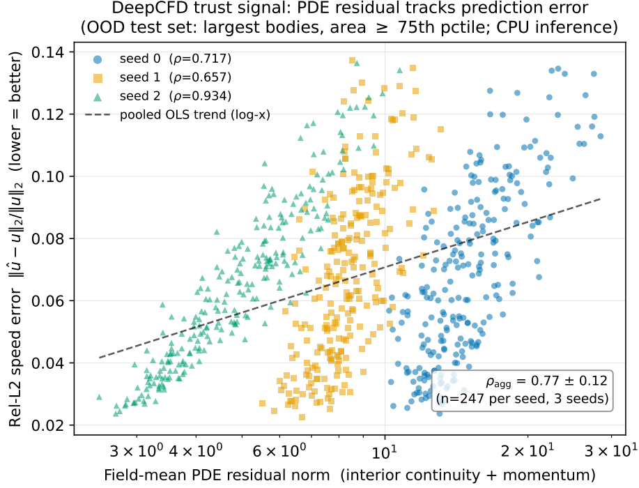
Figure 8: The trust signal generalizes to a second dataset (DeepCFD, 2-D laminar flow over bluff bodies; OOD held-out-largest-body split, 3 seeds). Per-case field-mean PDE residual norm (interior continuity+momentum) vs. rel- L_2 speed error: a low residual tracks a low error, as on AirFRANS. Per-case Spearman \rho = 0.77 \pm 0.12 (per seed 0.72/0.66/0.93; the trend holds within each seed—the colour-coded clusters span different residual ranges by initialisation). The residual is a reference-free error proxy on a geometry family and flow regime absent from AirFRANS.
