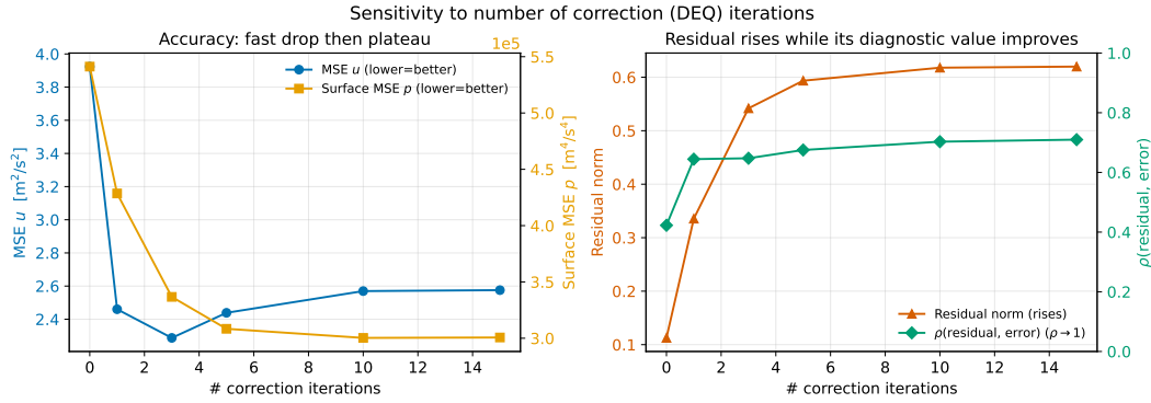
Figure 5: The money figure for the headline: PDE residual rises while field error falls across correction iterations (detector \neq fixer).
