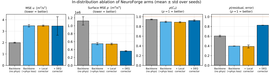
Figure 2: In-distribution ablation (Table 3): the DEQ corrector lifts the trust signal ( 0.40 \rightarrow 0.83 ) and surface fidelity while regressing volume \text{mse}_v/\text{mse}_p .
