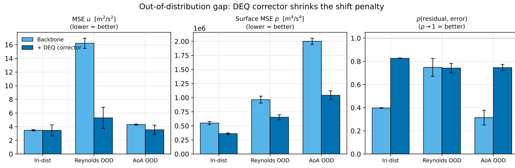
Figure 3: OOD gap and the regime-invariant trust signal ( \text{aoa} 0.31 \rightarrow 0.75 ); the bare backbone’s signal collapses, the corrected model’s holds.
