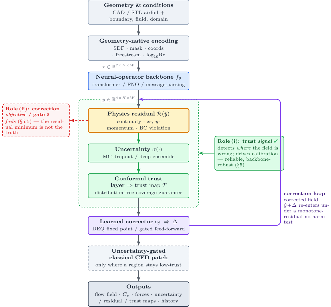
Figure 1: The NeuroForge pipeline. A one-shot neural-operator backbone f_\theta is wrapped in a verify–estimate–correct–fall-back loop. The physics residual \mathcal{R}(\hat{y}) (amber) is the pivot of the paper’s central dissociation : as a trust signal (role i, green) it reliably detects where the field is wrong and drives the uncertainty and distribution-free conformal layers, robustly across backbones; as a correction objective / acceptance gate (role ii, red) it fails, because the minimiser of the discrete residual is not the truth (subsection 5.5). The deployed correction is instead a learned corrector c_\phi (violet), whose corrected field re-enters under a monotone-residual no-harm test; it ingests the residual as one input channel, but a controlled ablation attributes its gain to the learned correction rather than to the residual input (subsection 5.2). Classical CFD is invoked only where a region remains low-trust. Tensor shapes follow the frozen 7-input/4-output channel contract.
