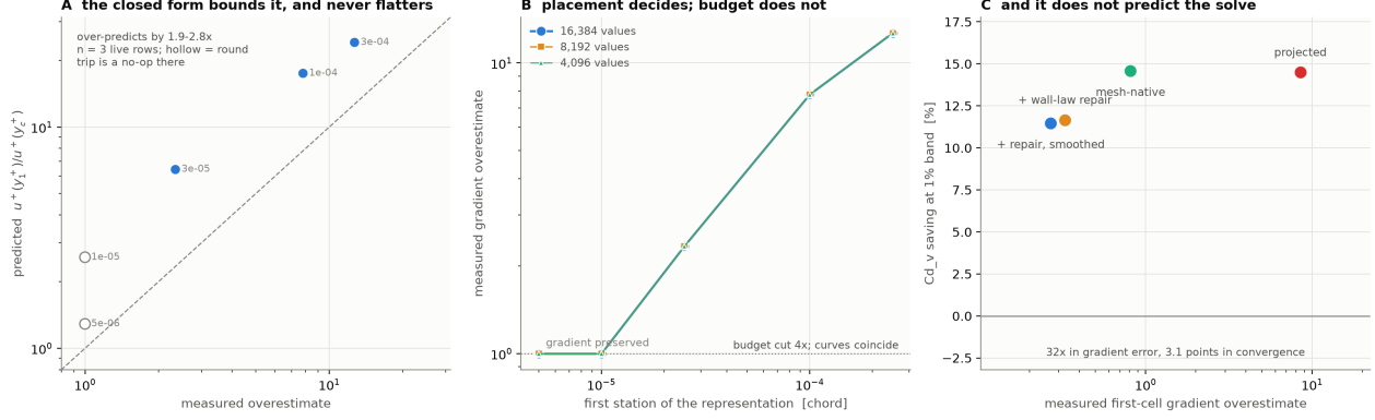
Figure 3. The criterion, what it controls, and what it fails to predict. (A) Predicted first-cell gradient overestimate against the measured one, at five first-station heights spanning a factor of fifty, with the identity line drawn. Every point sits above it — the expression is an upper bound and never flatters. The two hollow points are the rows where the round trip is a structural no-op (§6.2) and carry no information about the mechanism; the bound of 1.9–2.8 \times is claimed over the three filled ones. (B) The same measured damage against the first station’s height, one line per value budget. Cutting the budget fourfold, from 16,384 stored values to 4,096, leaves the three curves lying exactly on top of one another, while moving the station along the axis moves the damage 12.7 \times . Placement, not budget. (C) And none of it predicts the solve. Measured gradient error against C_{d,v} convergence saving, one point per arm: 32 \times in gradient error, 3.1 points in convergence. This panel is the paper’s negative result drawn, and §6.7 is what it means.
