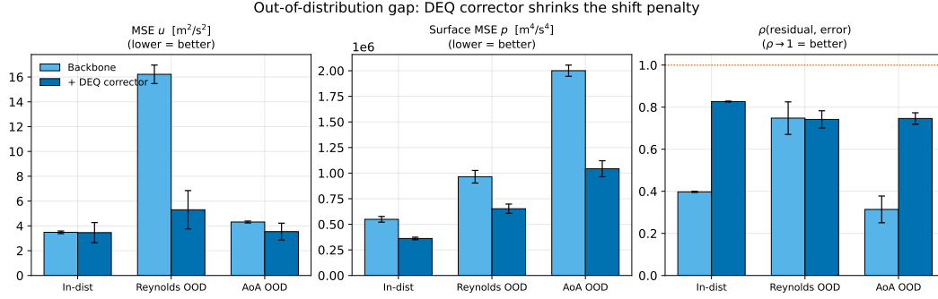
Figure 4: OOD gap and the regime-invariant trust signal ( aoa 0.31 \rightarrow 0.75 ); the bare backbone’s signal collapses, the corrected model’s holds.
