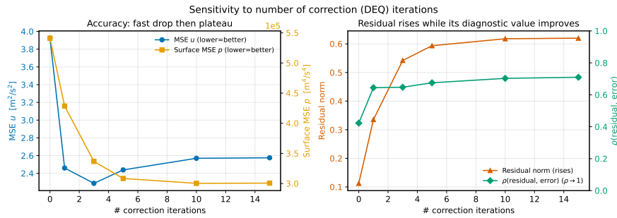
Figure 6: The iteration sweep (Table 10, one unseeded checkpoint). Over iterations 0 \rightarrow 3 the PDE residual rises while mse_u falls; beyond iteration 3 the two move together. A seeded five-seed re-run returns DIRECTION-ONLY, so this figure illustrates decoupling between the residual and the error, not divergence. The claim itself rests on subsubsection 5.9.2 .
