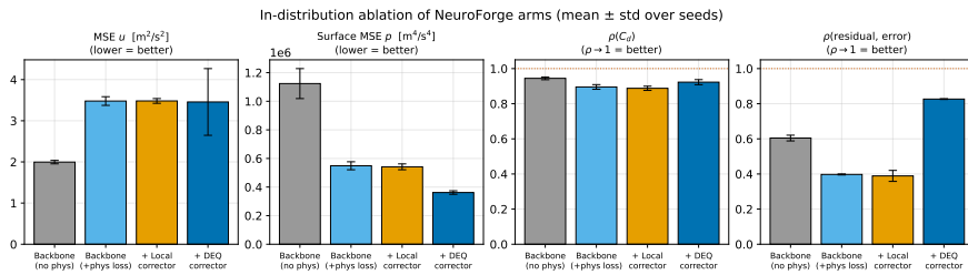
Figure 3: In-distribution ablation (Table 8): the DEQ corrector lifts the trust signal ( 0.40 \rightarrow 0.83 ) and surface fidelity while regressing volume mse_v/mse_p .
