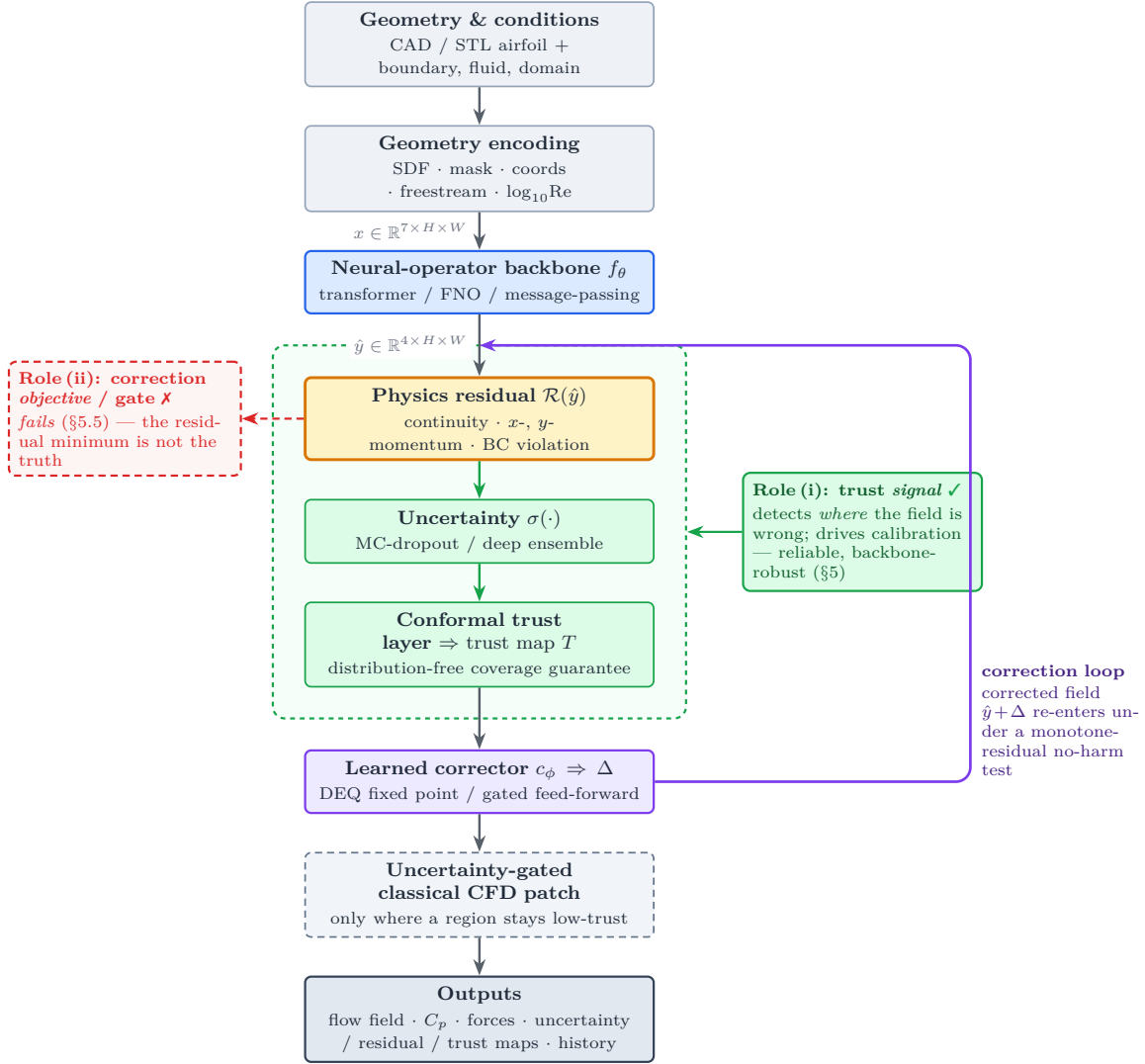
Figure 1: The NeuroForge pipeline. A one-shot backbone f_\theta is wrapped in a verify–estimate–correct–fall-back loop. Colour marks each component’s role: the physics residual (amber) acts as a reliable trust signal (role i, green) but not as a correction objective/gate (role ii, red); the deployed correction is a learned corrector (violet) applied under a monotone-residual no-harm test. The two roles, and the attribution of the corrector’s gain, are established and scoped in the text (section 3, section 5).
