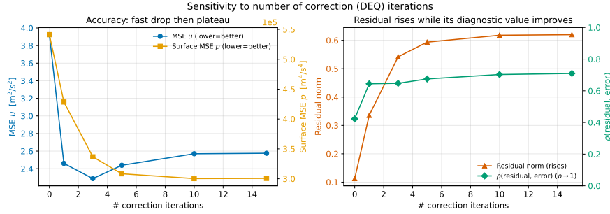
Figure 6: The iteration sweep that first prompted the question (Table 6, one unseeded checkpoint). Over iterations 0 \rightarrow 3 the PDE residual rises while mse_u falls; beyond iteration 3 the two move together. A seeded five-seed re-run returns DIRECTION-ONLY, so this figure illustrates decoupling between the residual and the error, not divergence. The claim itself rests on subsection 5.7.
