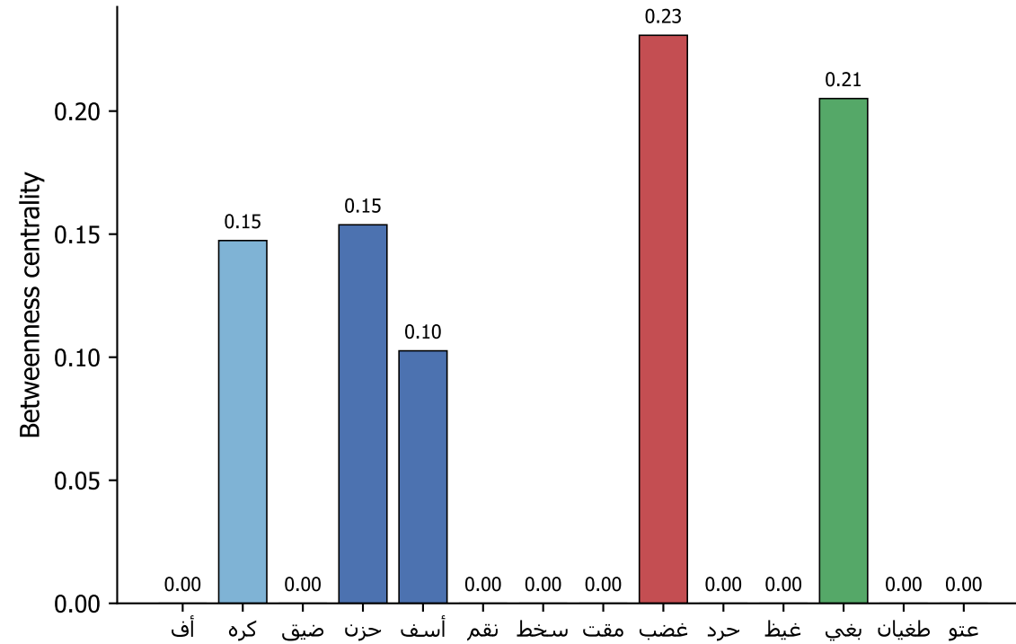
(b) Betweenness centrality (bridge-node strength)
