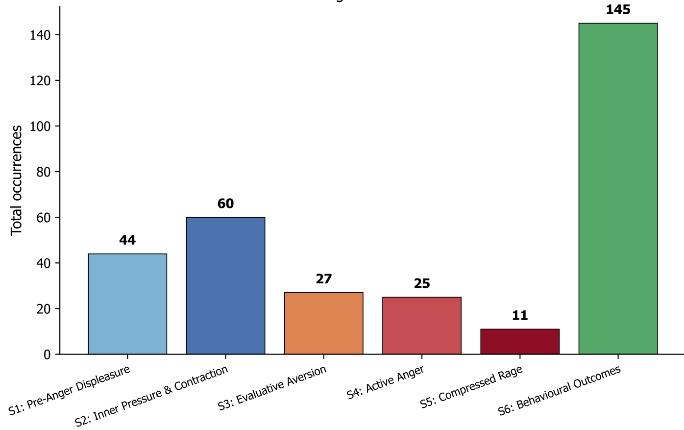
Stage-level totals
