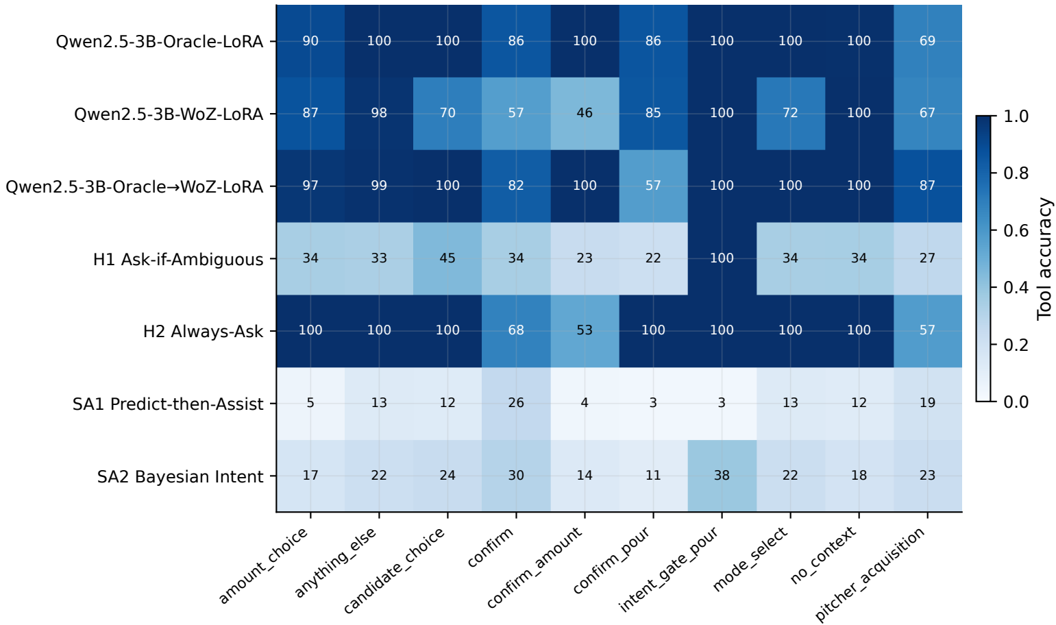
Tool accuracy by dialog context — oracle_valid_pouring
