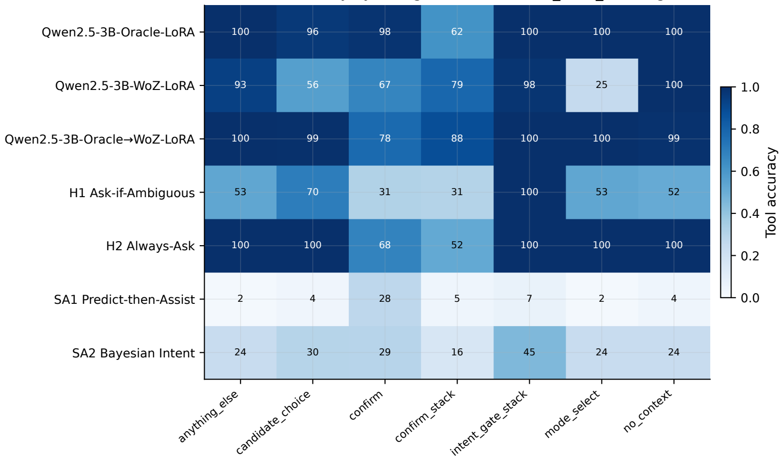
Tool accuracy by dialog context — oracle_valid_stacking
