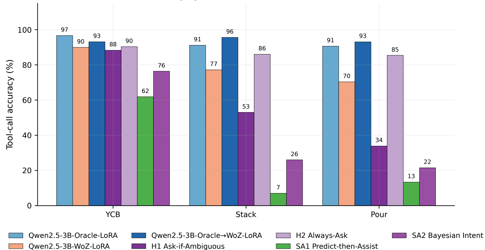
Tool-call accuracy by environment (oracle held-out validation)
