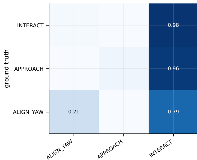
Qwen2.5-3B-WoZ-LoRA
