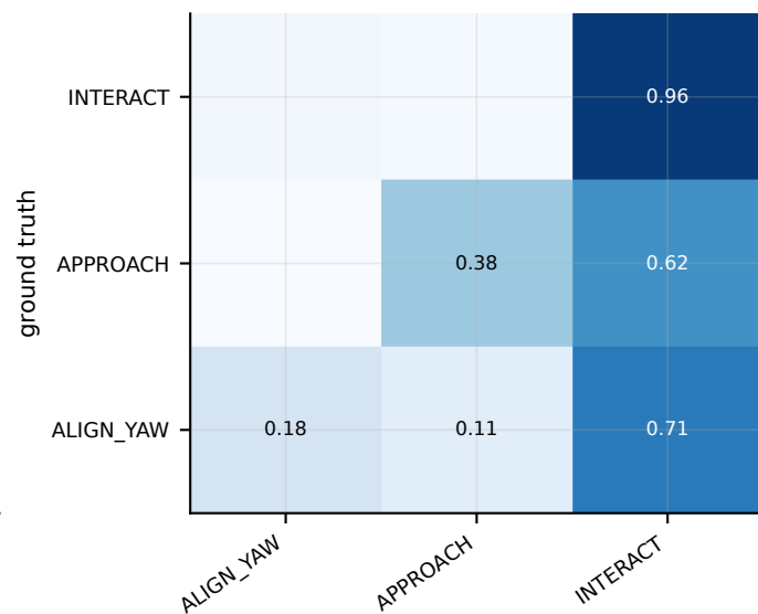
Qwen2.5-3B-WoZ-LoRA
