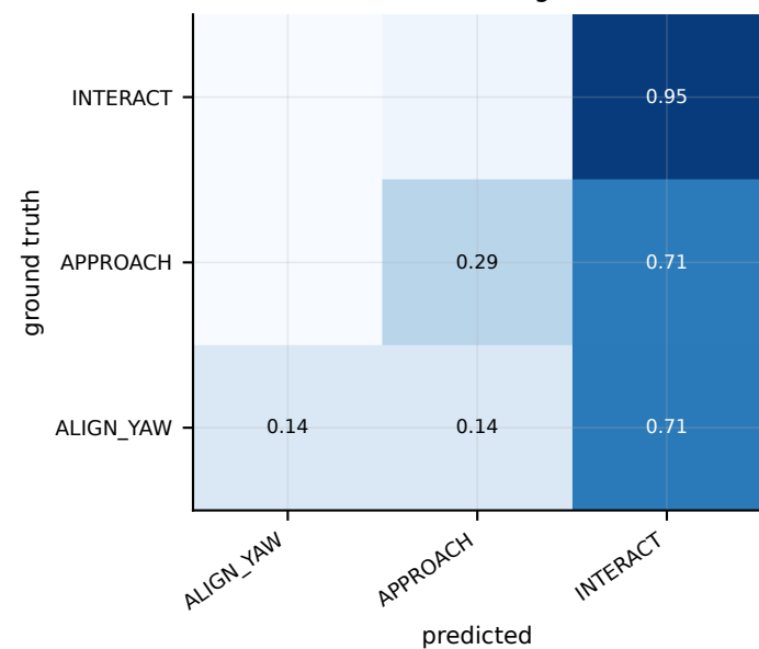
H1 Ask-if-Ambiguous
