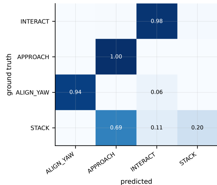
H1 Ask-if-Ambiguous
