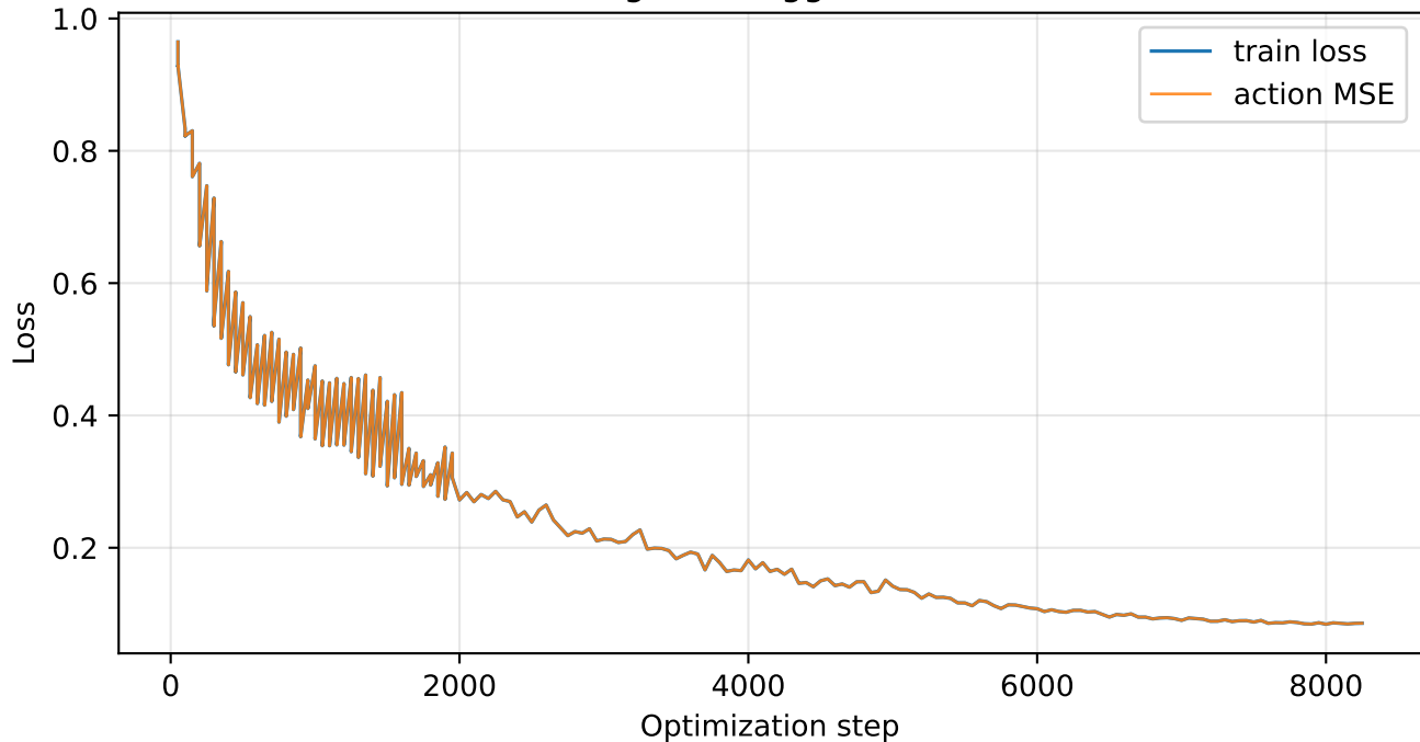
Training loss (logged batches)
