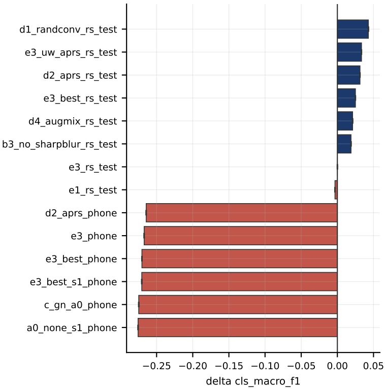
cls_macro_f1 relative to e3_rs_test
