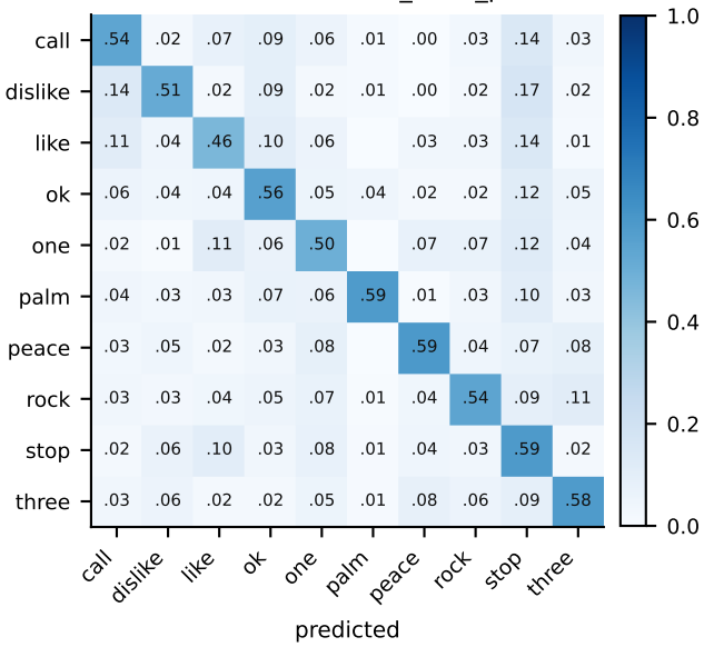
confusion matrix — a0_none_pseudo
