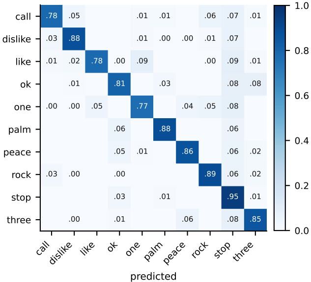
confusion matrix — a0_none_rs_test
