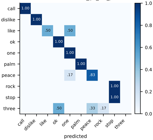
confusion matrix — e3_gn_uw_phone
