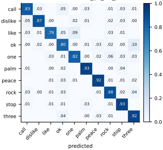
confusion matrix — e3_gn_uw_pseudo
