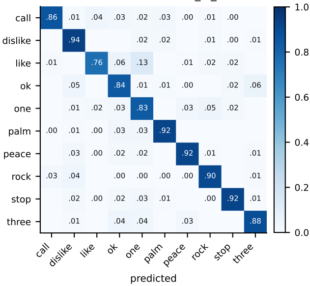
confusion matrix — e3_rs_test
