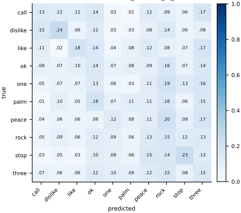
confusion matrix — b0_classical_rs_test
