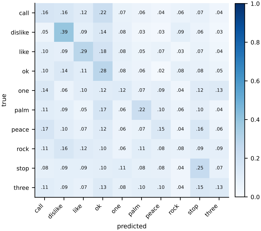
confusion matrix — b0_classical_rs_val
