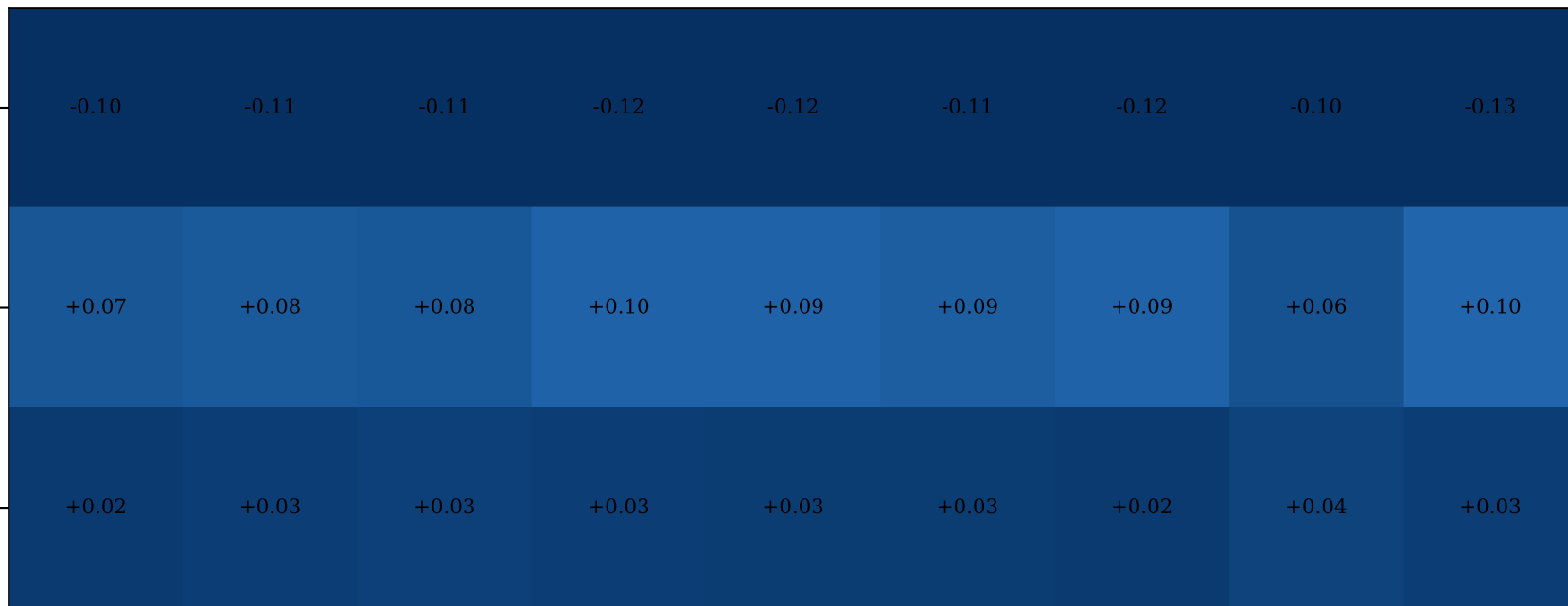
Difference Heatmap: \rho_{\text{hardware}} - \rho_{\text{Trotter}}
