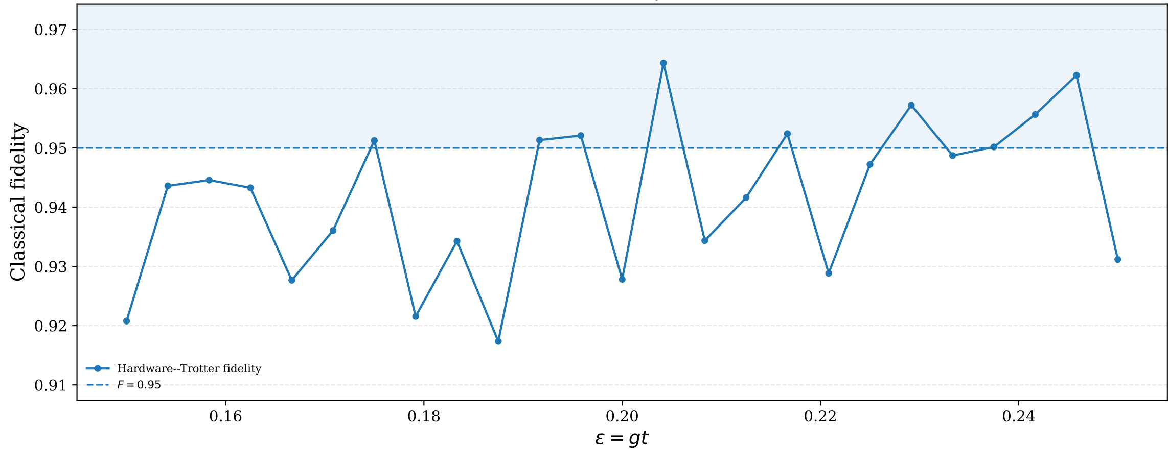
Hardware--Trotter Fidelity (20 Trotter steps)
