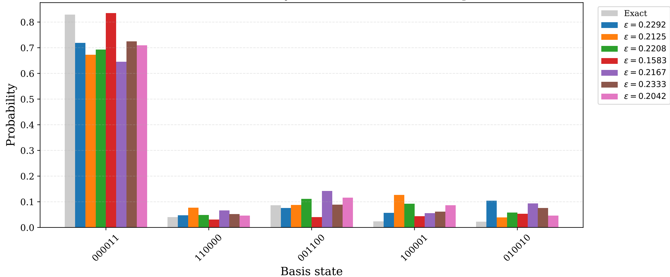
Postselected Probability Distributions (5 Trotter steps)
