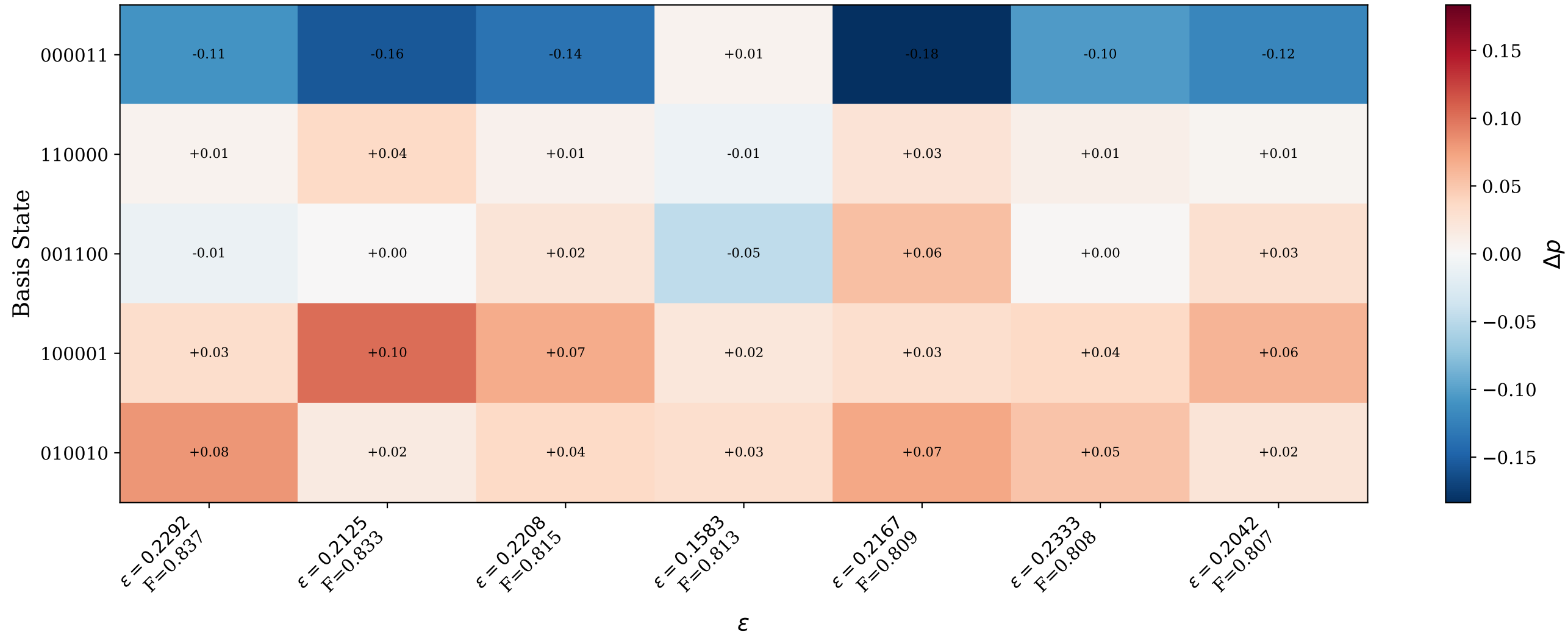
Difference Heatmap: \rho_{\text{hardware}} - \rho_{\text{exact}}
