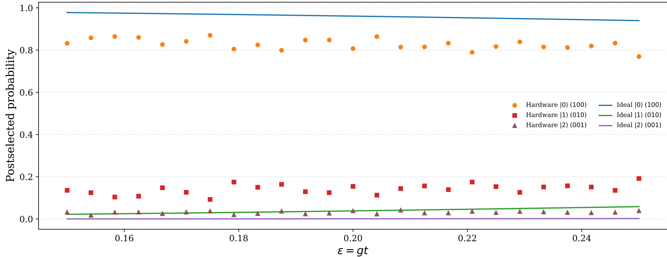
Single-Excitation State Populations (20 Trotter steps)
