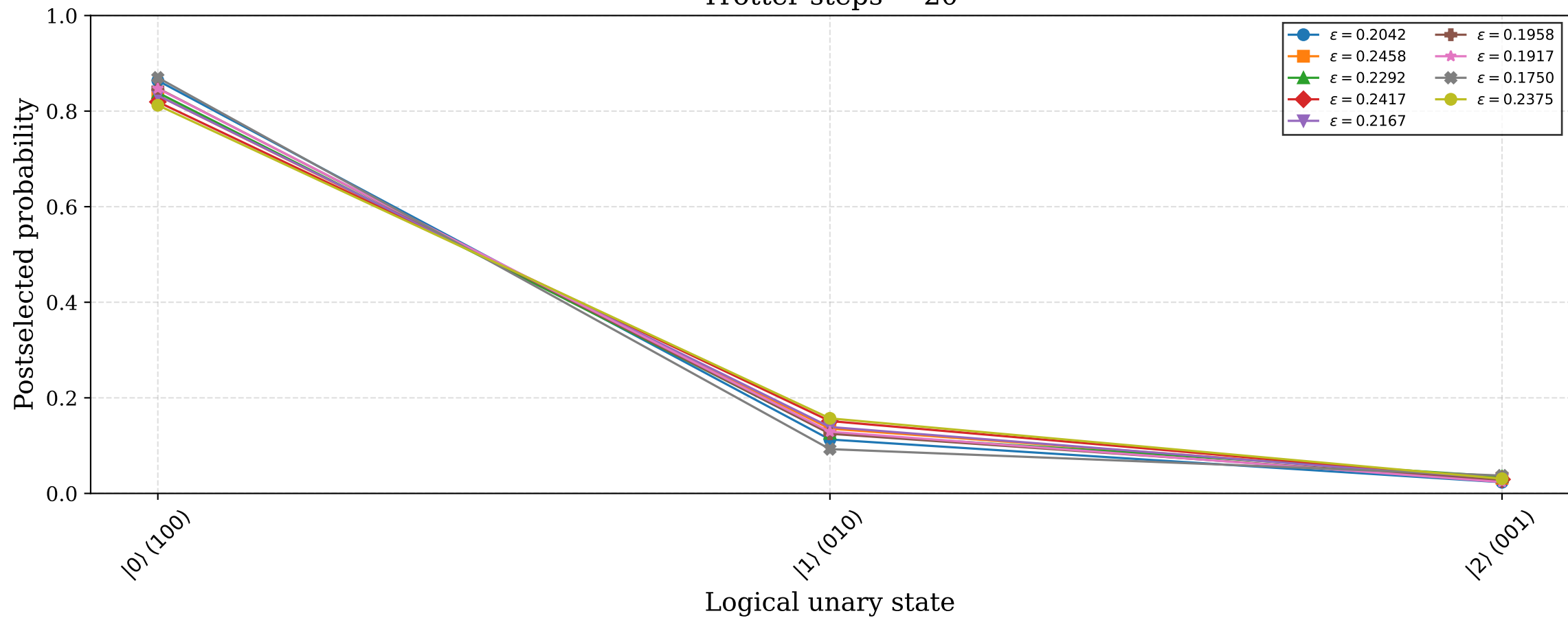
Trotter steps = 20
