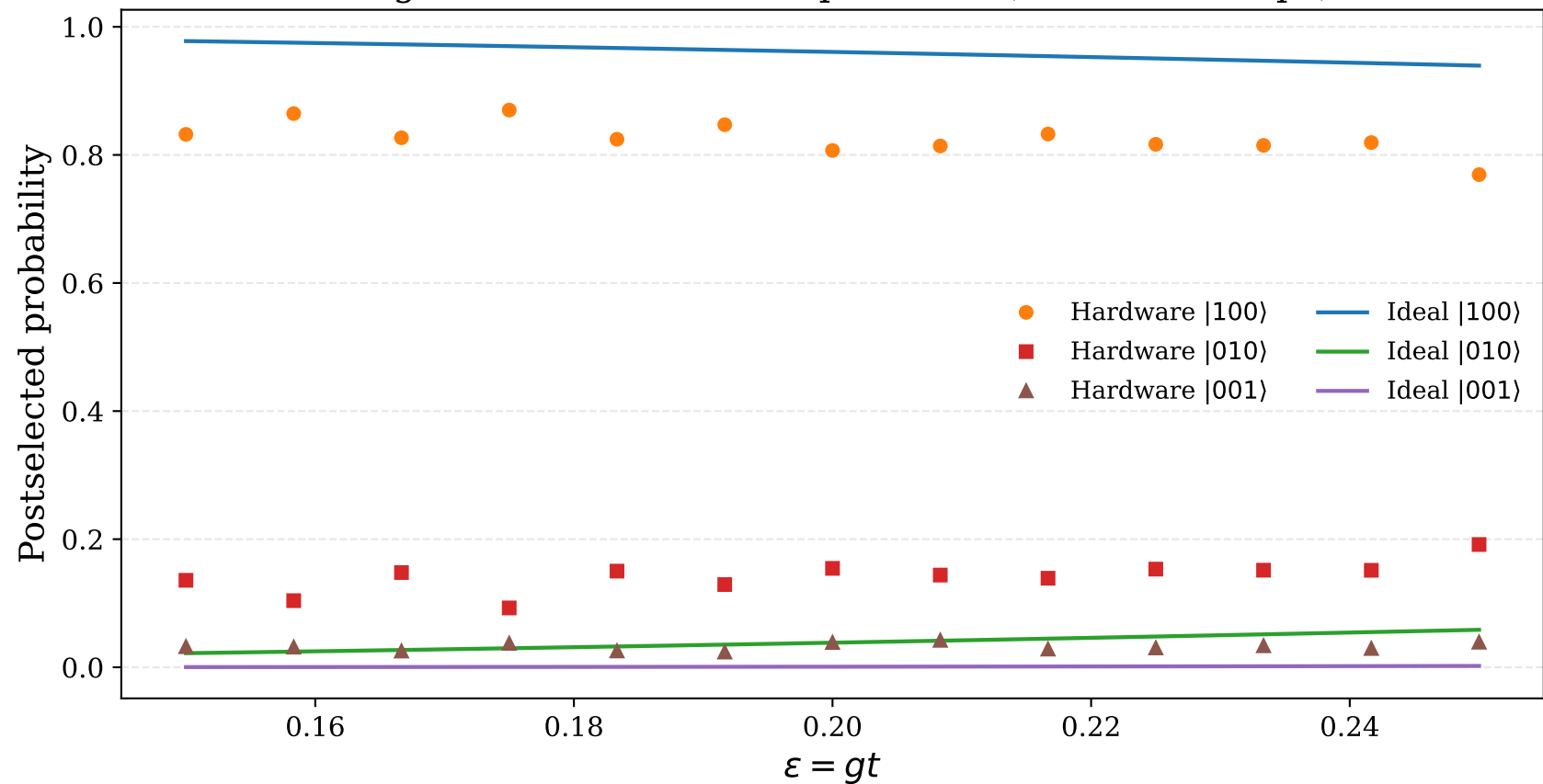
Single-Excitation State Populations (20 Trotter steps)
