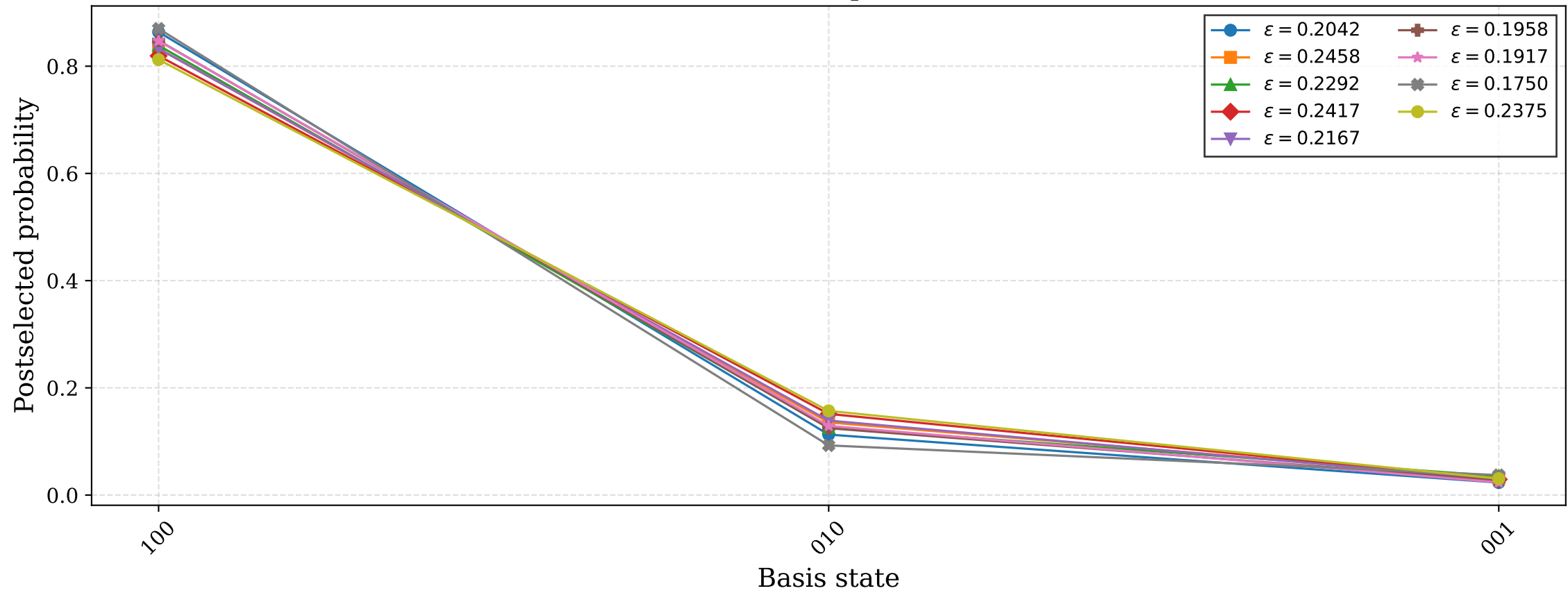
Trotter steps = 20
