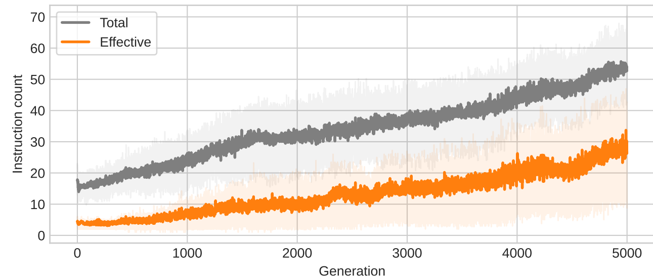
Fixed Mutation Rates
