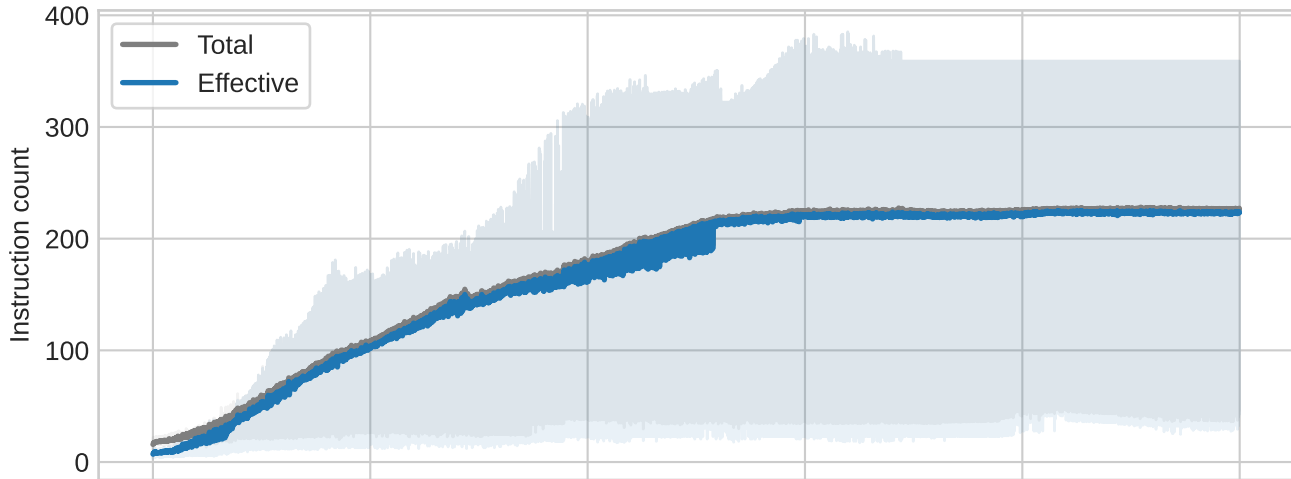
Fixed Individual Mutation Rates
