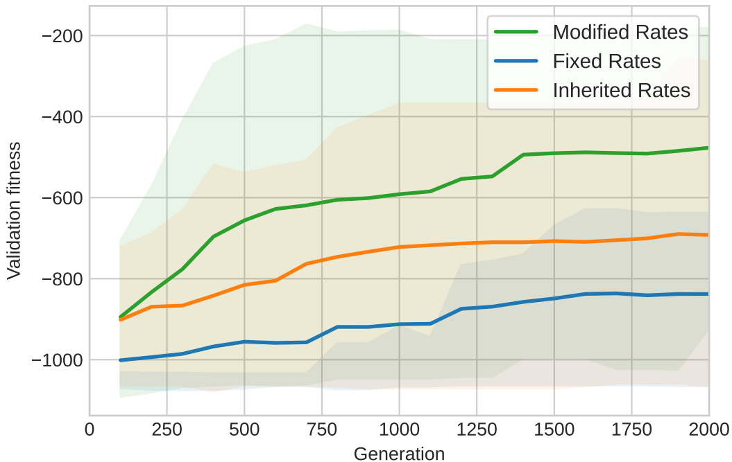
Pendulum Task: Validation fitness
