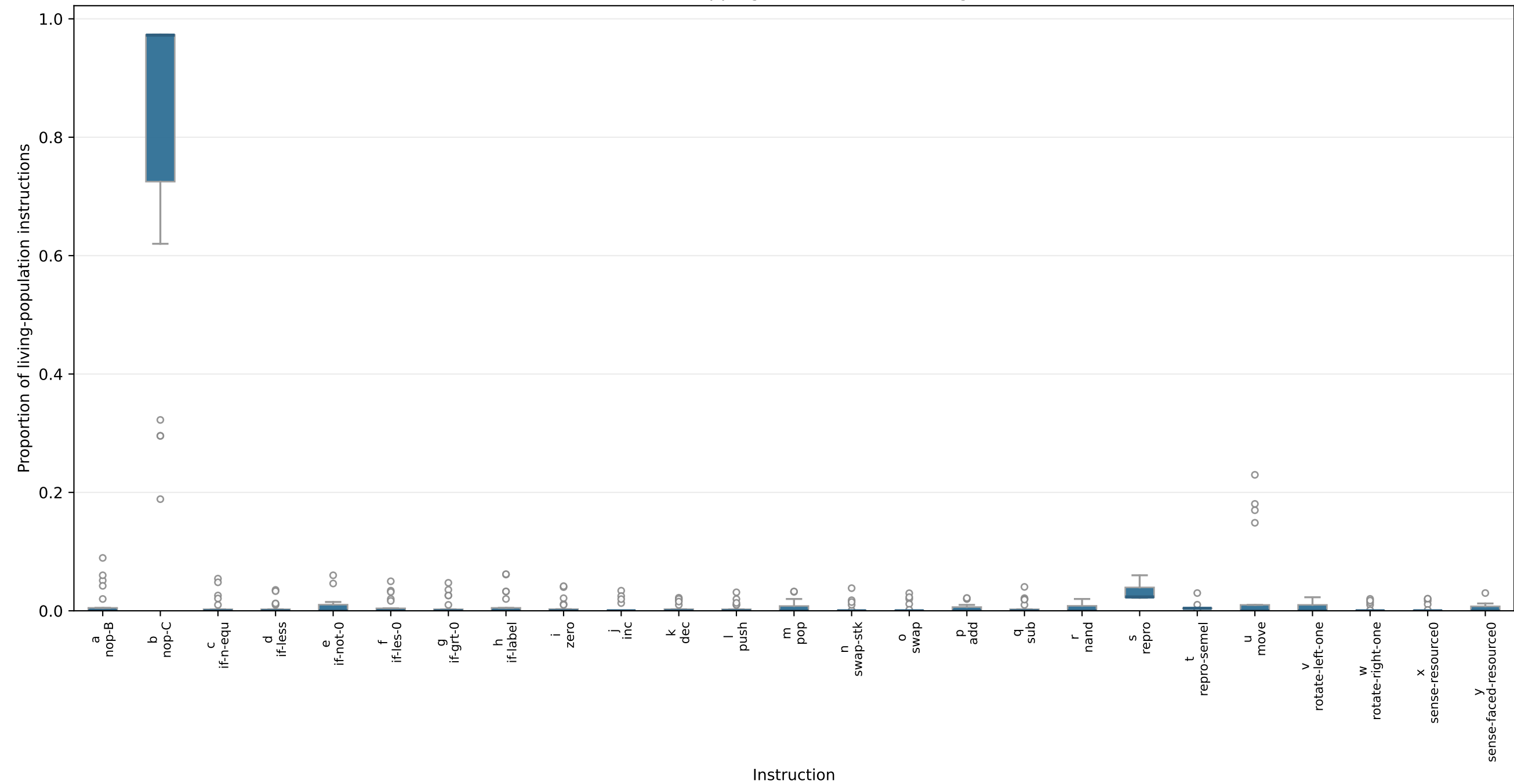
Non-overlapping 1000 instruction usage
