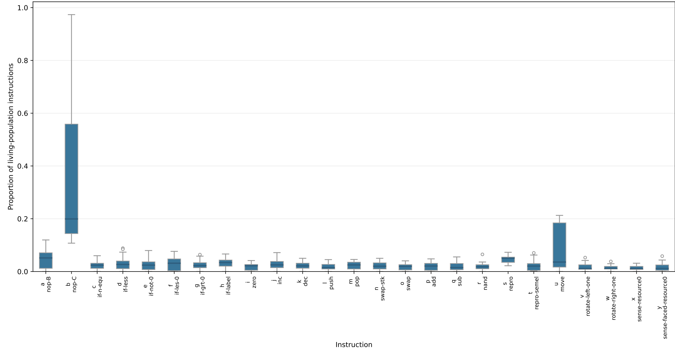
Overlapping 500 instruction usage
