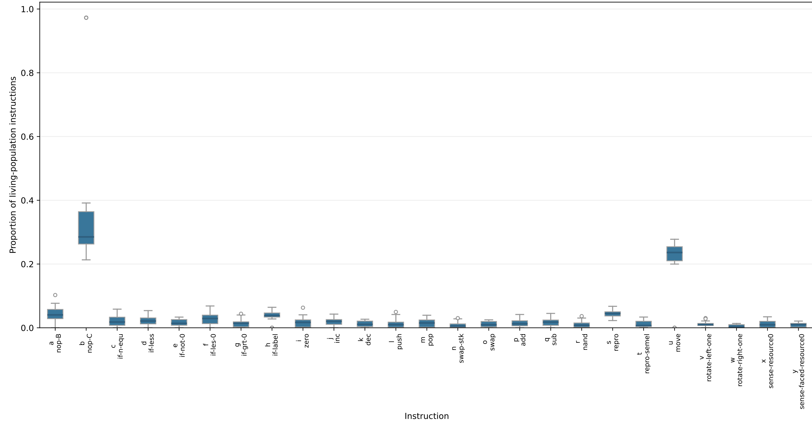
Non-overlapping 1000 RC instruction usage
