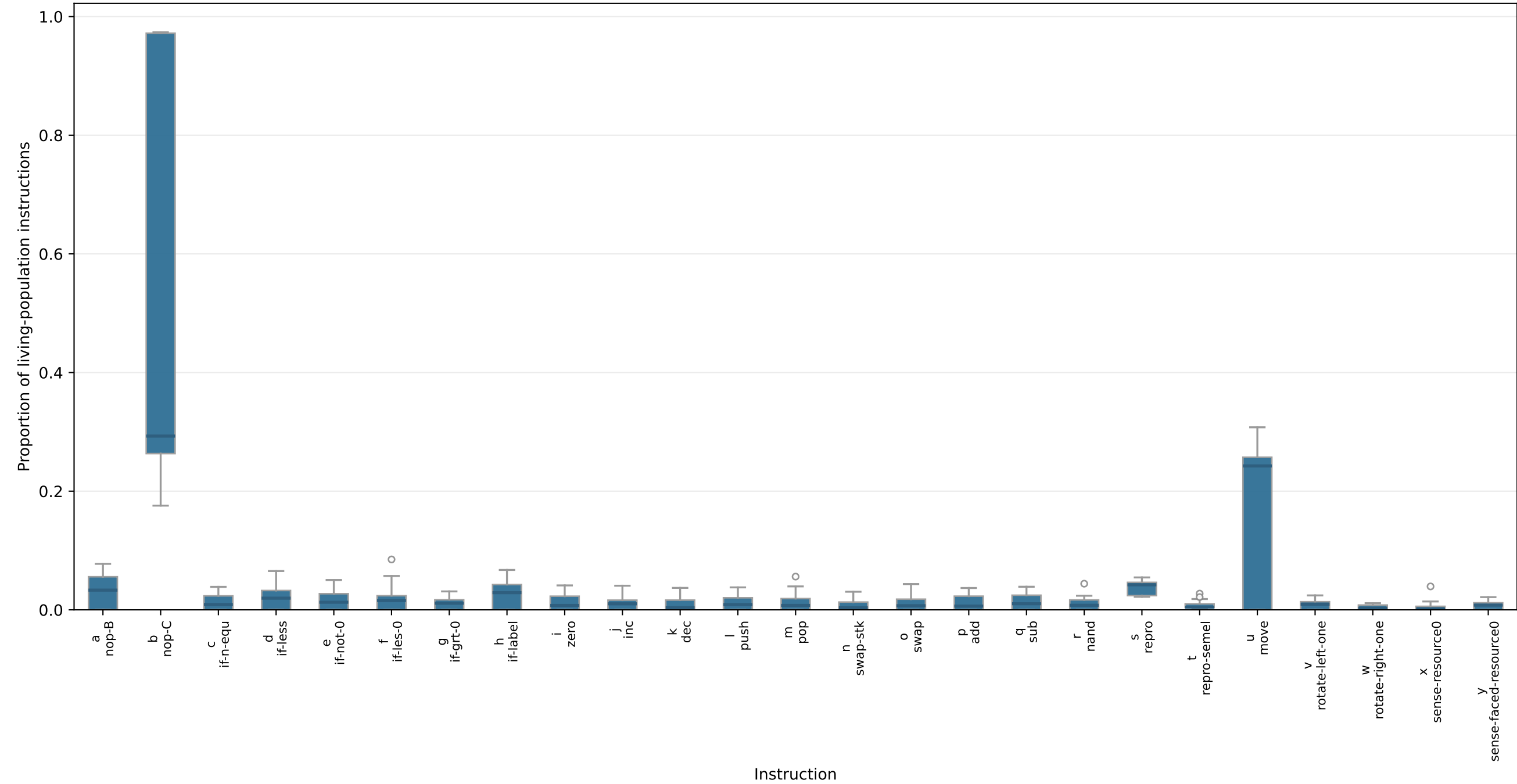
Non-overlapping 500 RC instruction usage
