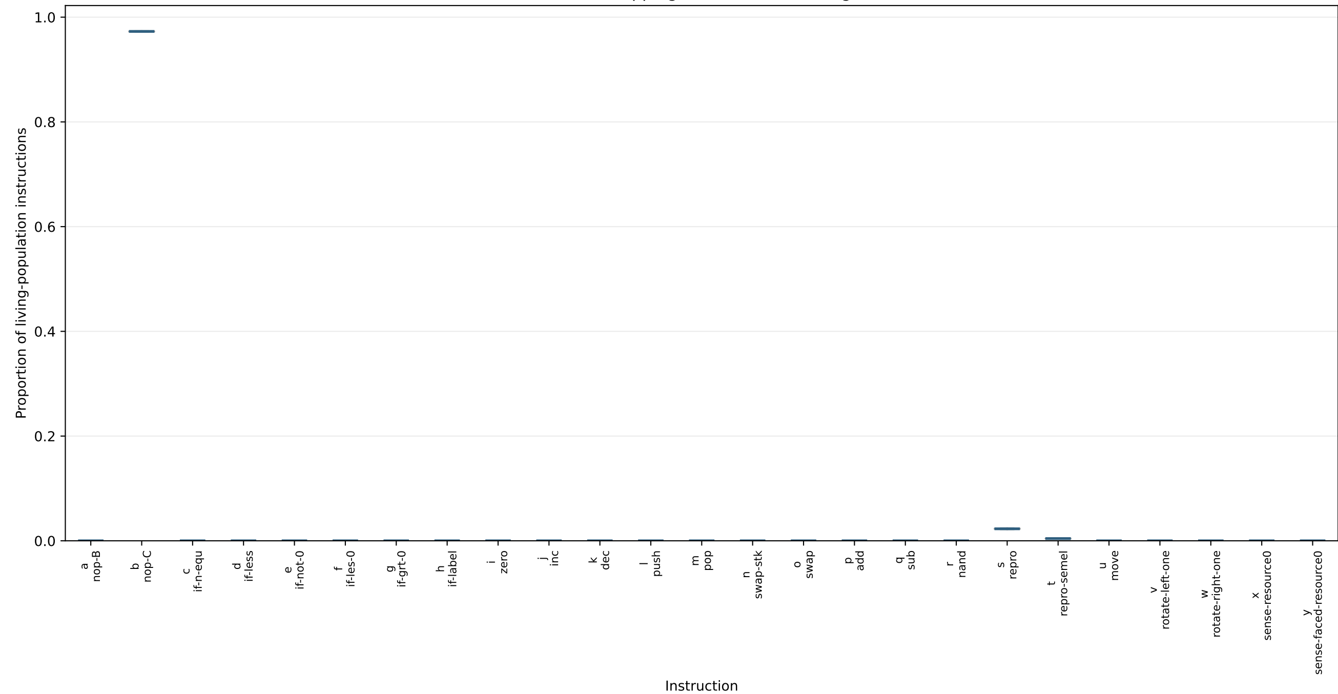
Non-overlapping 200 instruction usage
