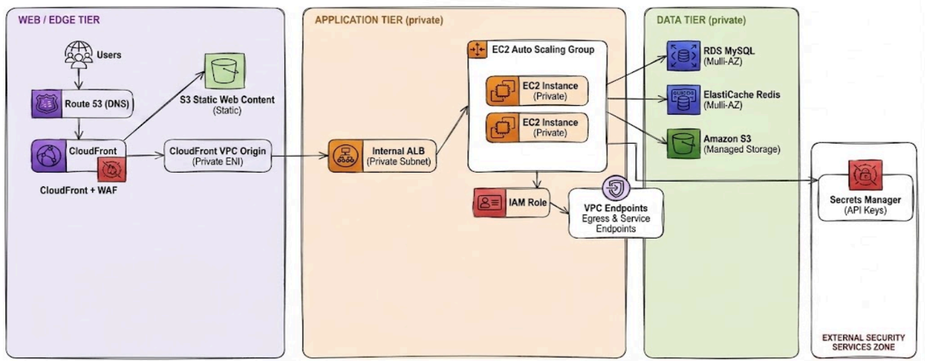
Figure 1 — High-level AWS architecture
