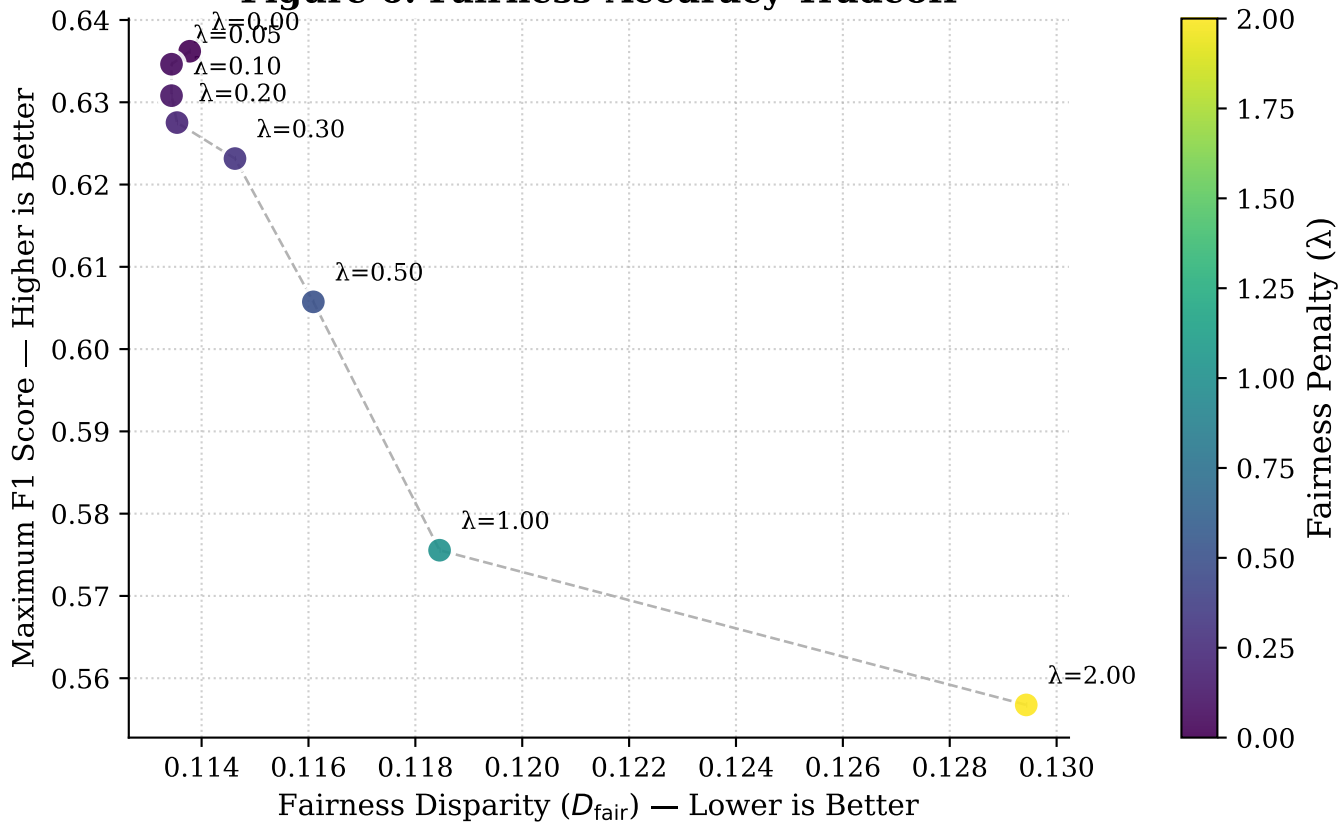
Figure 6: Fairness-Accuracy Tradeoff
